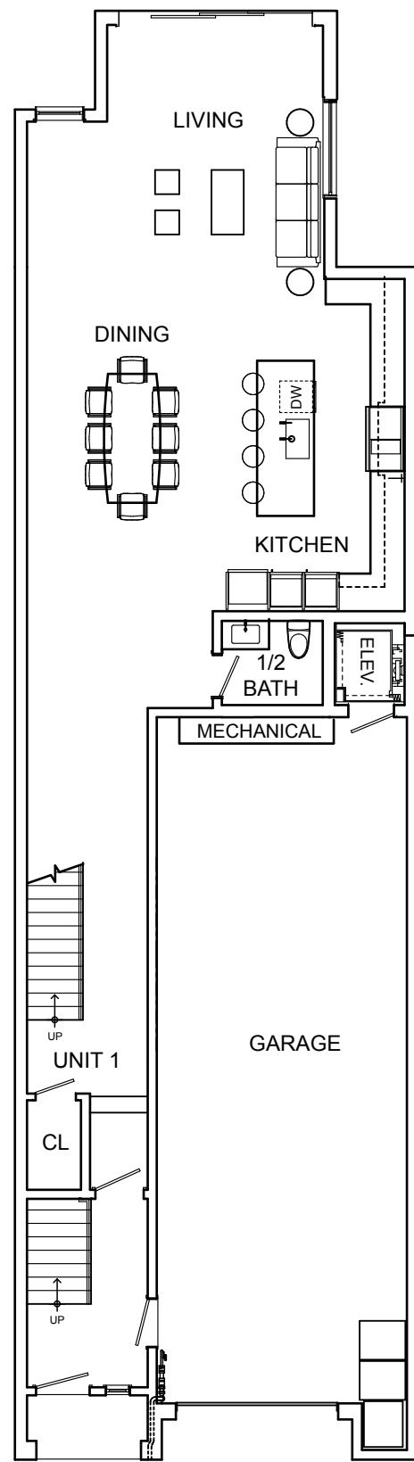
FIRST FLOOR
